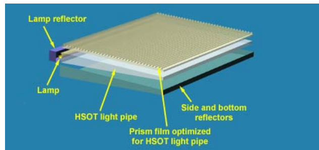
Picture 9. Example of HSOT light pipe device.
