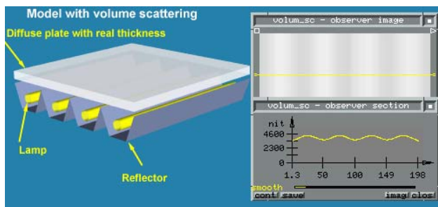
Picture 8. Accurate simulation of Volume Scattering effect.
